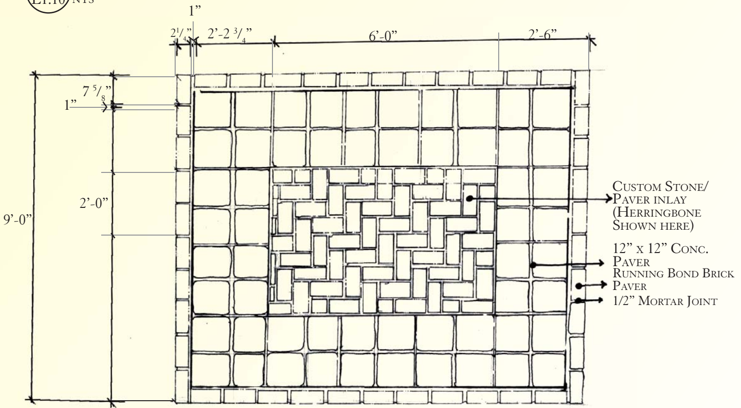
2 PLAN VIEW OF BRICK & CONCRETE PATIO L1.10 NTS
