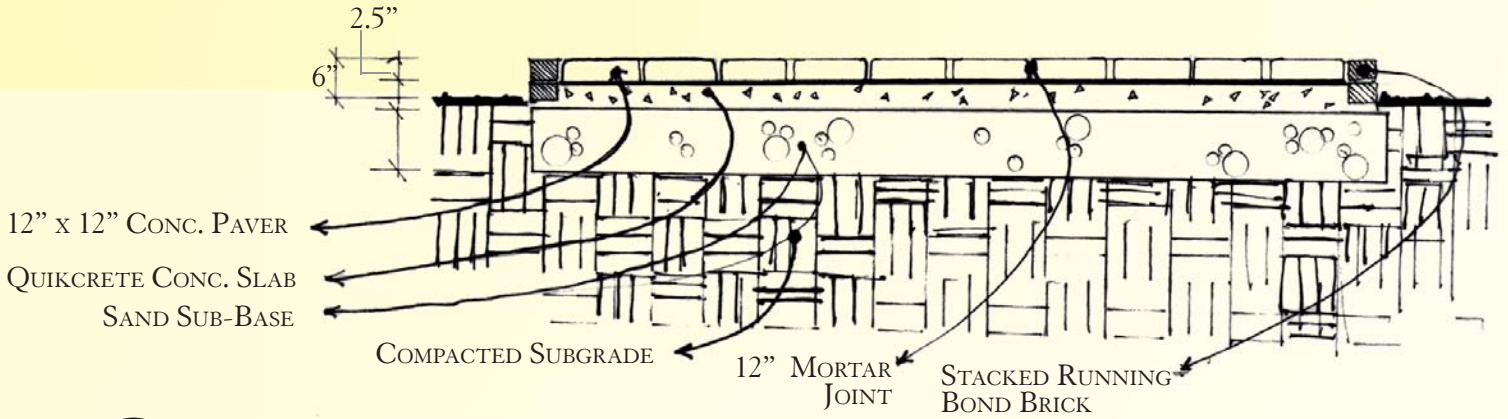
1 SECTION OF BRICK & CONCRETE PATIO L1.10 NTS
