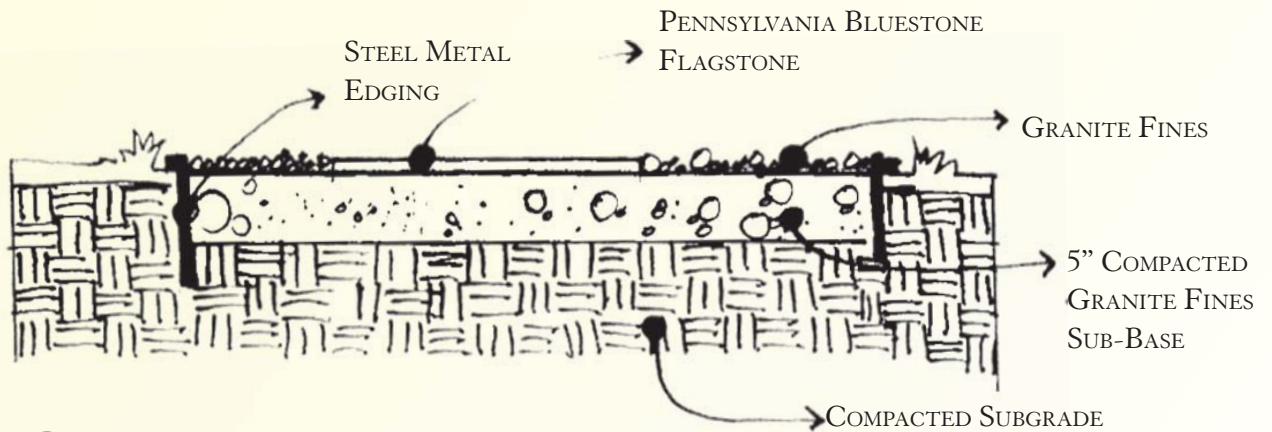
2 SECTION VIEW OF FLAGSTONE PATH L1.6 NTS
